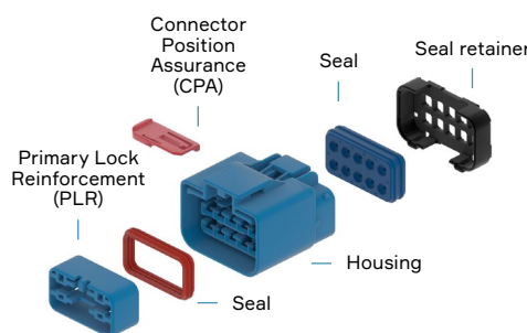
APEX® 2.8 Sealed 10W Female
